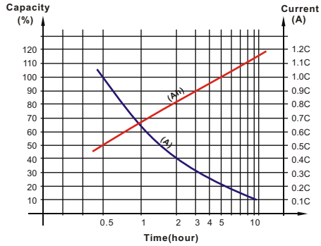
Discharge Characteristics
