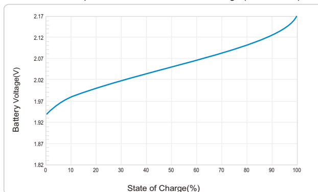
Relationship of OCV and State Of Charge ( 25^{\circ}C, 77^{\circ}F )
