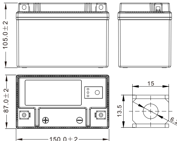
Dimensions (mm)
